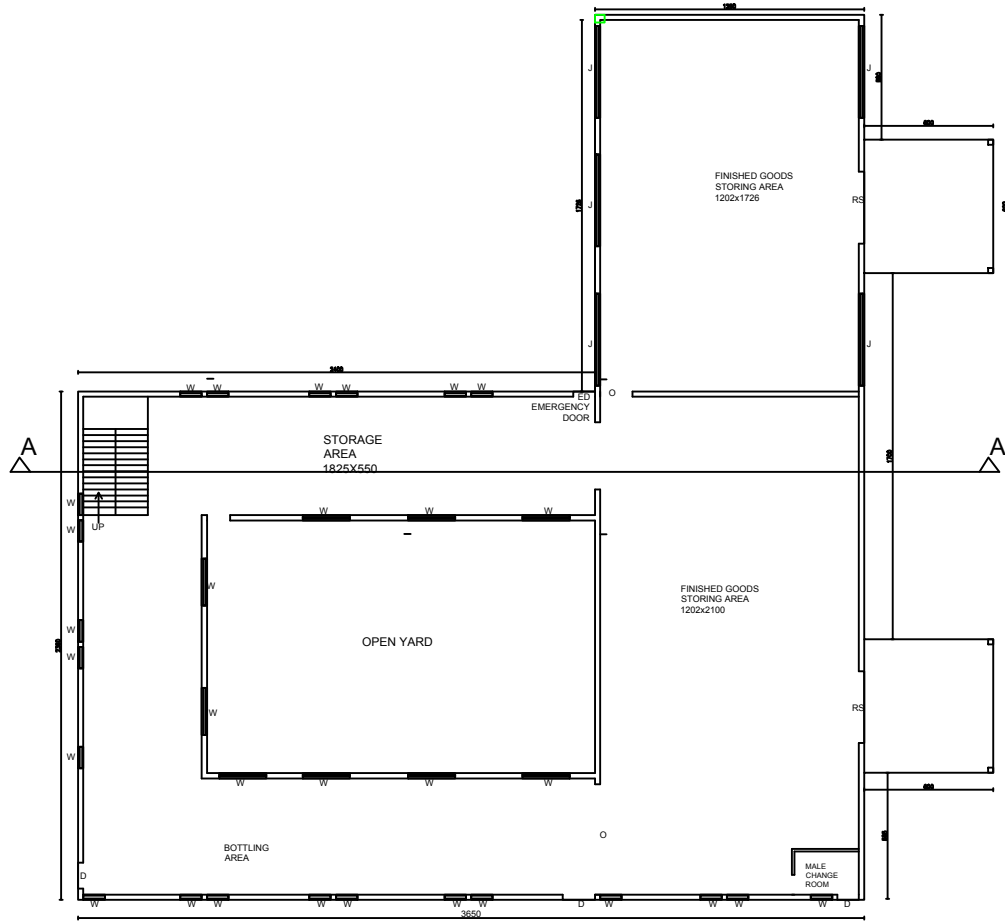
GROUND FLOOR PLAN OF ARISHTAM BOTTLING PLANT
