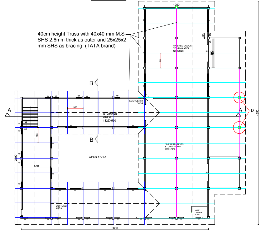
FIRST FLOOR PLAN OF ARISHTAM BOTTLING PLANT
